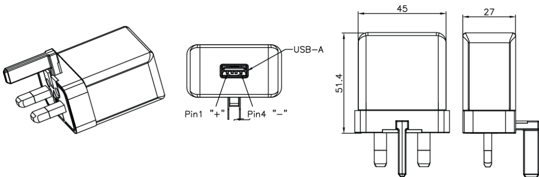
PSA15K-308Q-H Dimension Diagram Unit: mm
