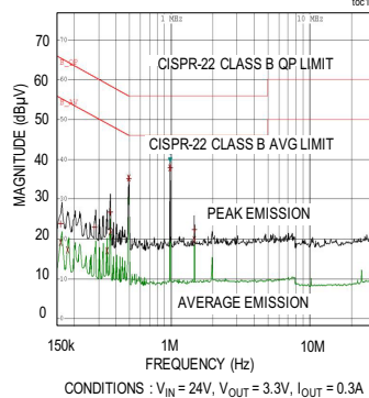
CONDUCTED EMISSION PLOT (EMI FILTER: C6, C7 = 0.1μF, C8 = 0.47μF, L1 = 82μH, C9 = 1μF)
