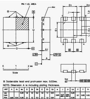
DFN2020MD-6 (SOT1220)
