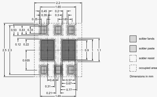
DFN2020D-6 (SOT1118D)
