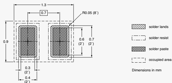
DFN1006-2 (SOD882)
