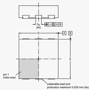
DFN2020D-6 (SOT1118D)
