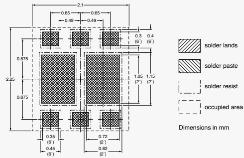
DFN2020-6 (SOT1118)
