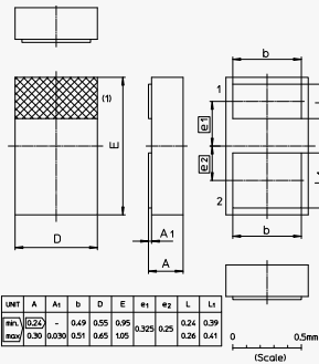
DSN1006U-2 (SOD995)
