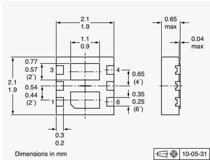
DFN2020-6 (SOT1118)
