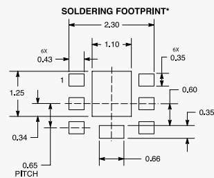
DFN2020MD-6 (SOT1220)
