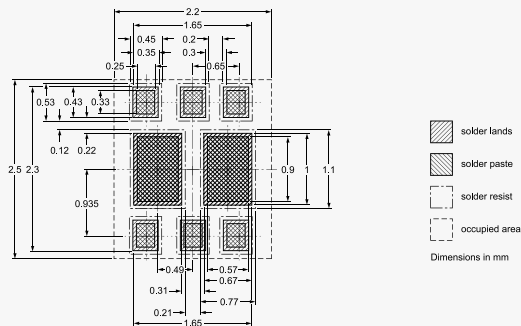
DFN2020D-6 (SOT1118D)
