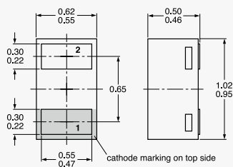
DFN1006-2 (SOD882)
