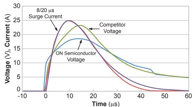
Line-to-Line Surge
