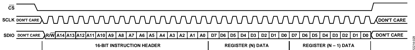
Figure 32. Serial Control Port Write—MSB First, Address Decrement, Two Bytes of Data
