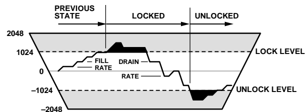
Figure 29. Lock Detector Diagram
