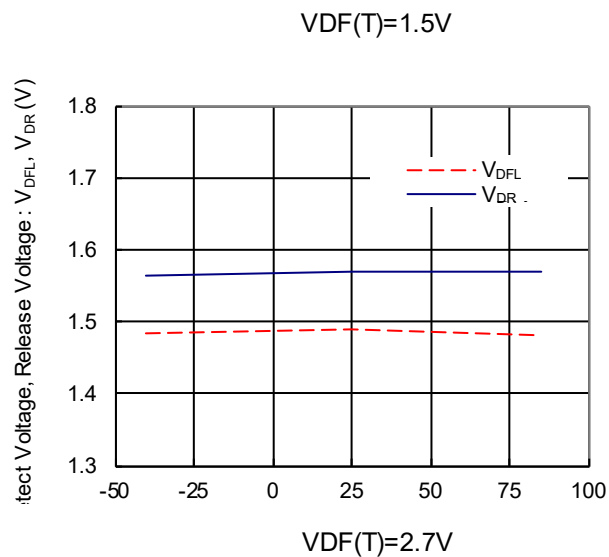
(4) Detect Voltage, Release Voltage vs. Ambient Temperature
