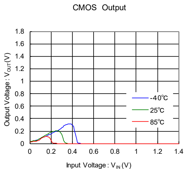
(6) Output Current (Nch Driver) vs. Input Voltage
