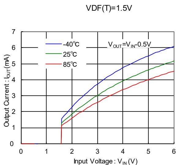
(7) Output Current (Pch Driver) vs. Input Voltage
