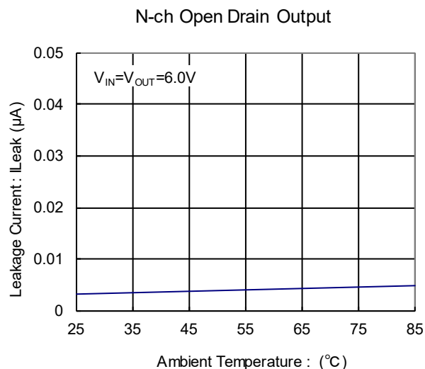
(8) Leakage Current vs. Ambient temperature
