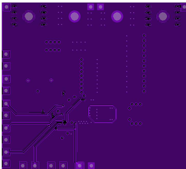
Fig. 5: Board Layout-Mid Layer 2
