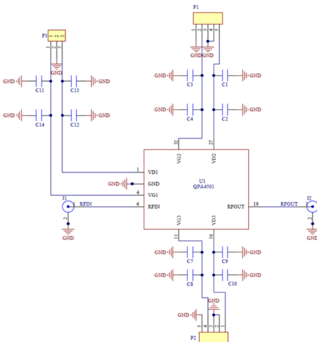
EVB Schematic
