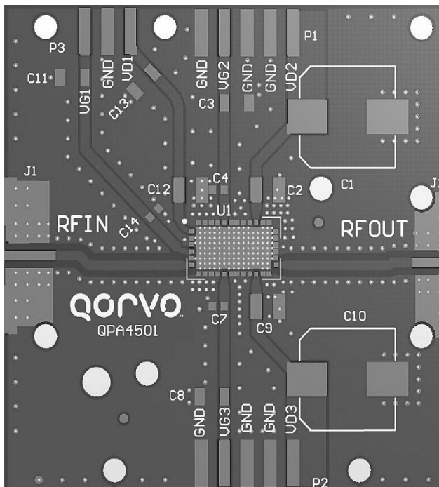
EVB Layout
