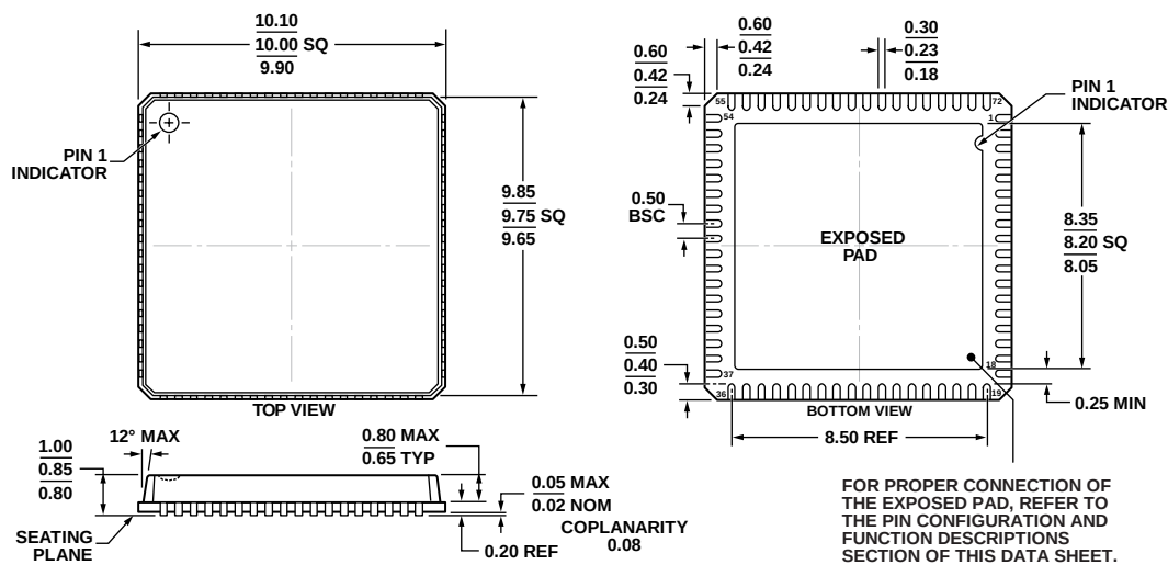
Figure 65. 72-Lead Lead Frame Chip Scale Package [LFCSP_VQ] 10 mm x 10 mm Body, Very Thin Quad (CP-72-3) Dimensions shown in millimeters
