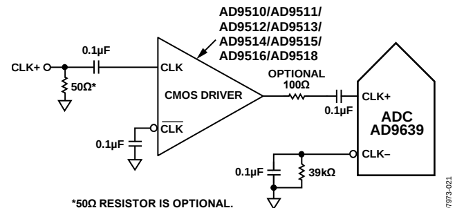
Figure 46. Single-Ended 1.8 V CMOS Sample Clock
