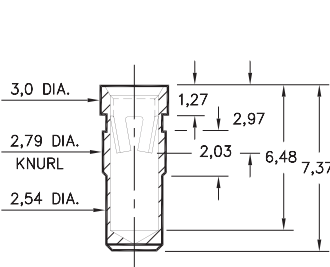
5834-0-15-XX-23-XX-10-0 Press-fit in 2,72 mounting hole
