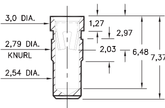
5834-0-15-XX-23-XX-10-0 Press-fit in 2,72 mounting hole
