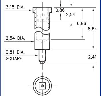
4582-0-15-XX-23-XX-10-0 Square press-fit in 1,02 plated thru hole
