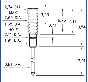
1105-0-15-XX-13-XX-04-0 Press-fit in 2,03 mounting hole
