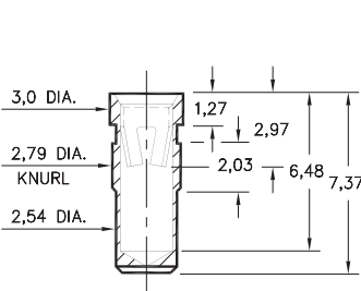
5834-0-15-XX-23-XX-10-0 Press-fit in 2,72 mounting hole
