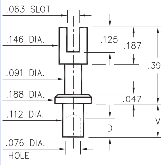
2809-X-01-XX-00-00-07-0 Swage mount in .116 hole
