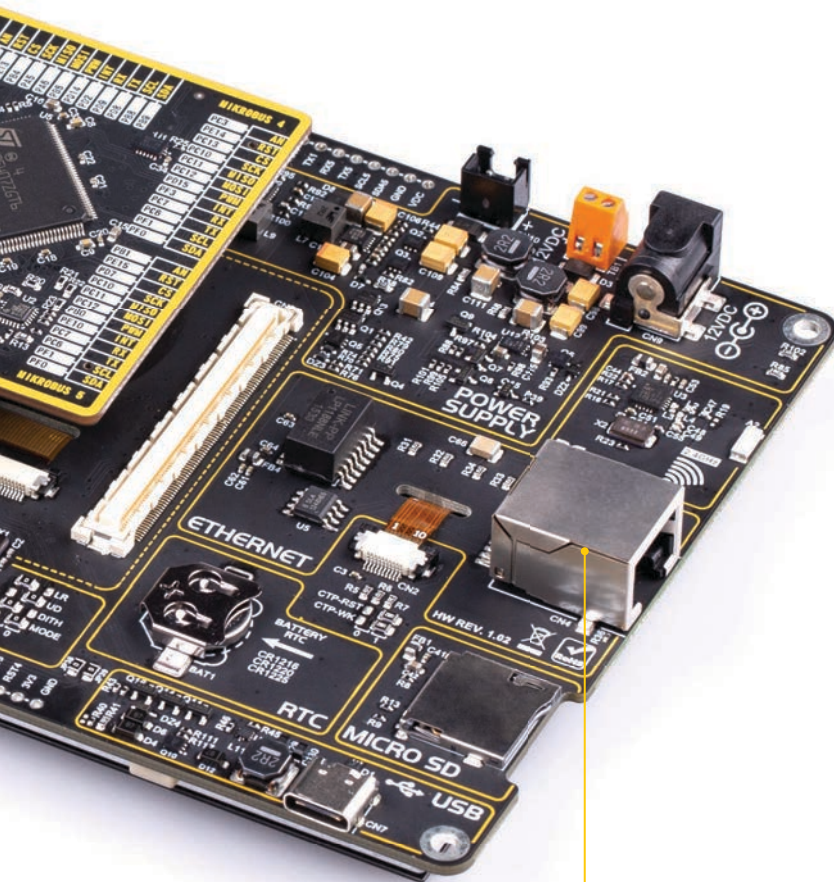
Figure 12: RJ-45 connector view
