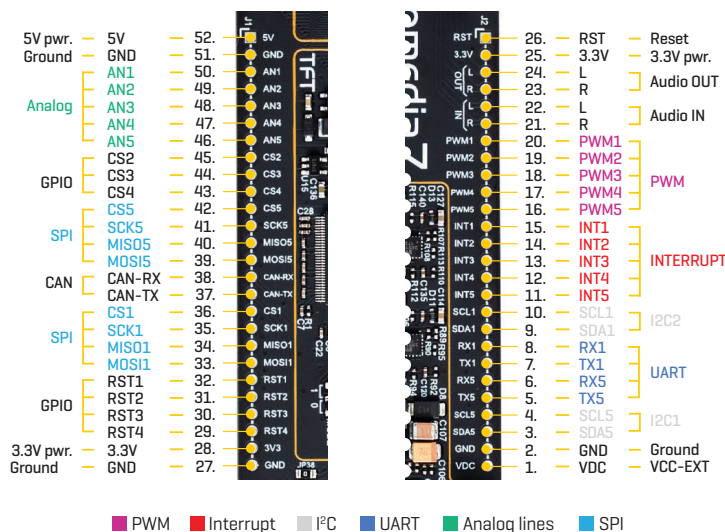
Figure 15: 1x26 pin header view
