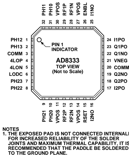
Figure 2. 32-Lead LFCSP Pin Configuration
