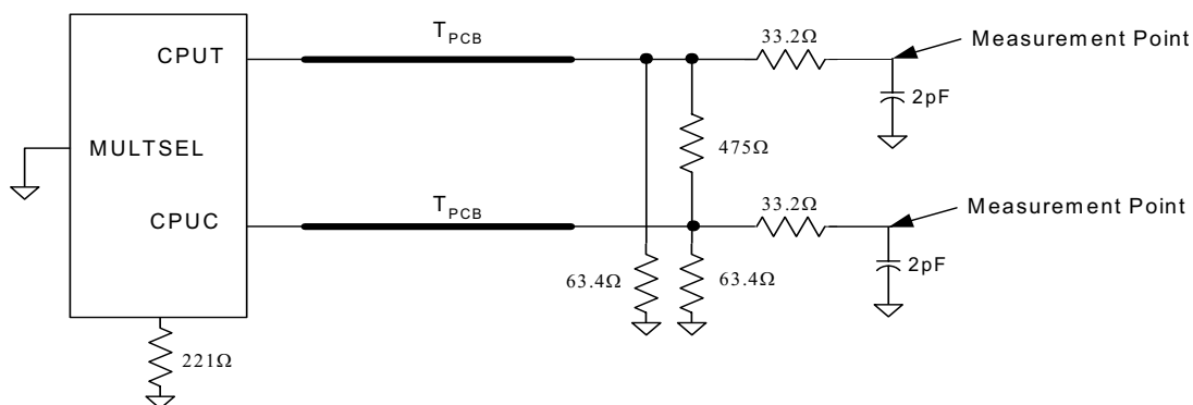
Figure 11. 1.0V Test Load Termination
