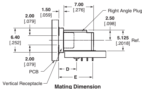
Mating Dimension
