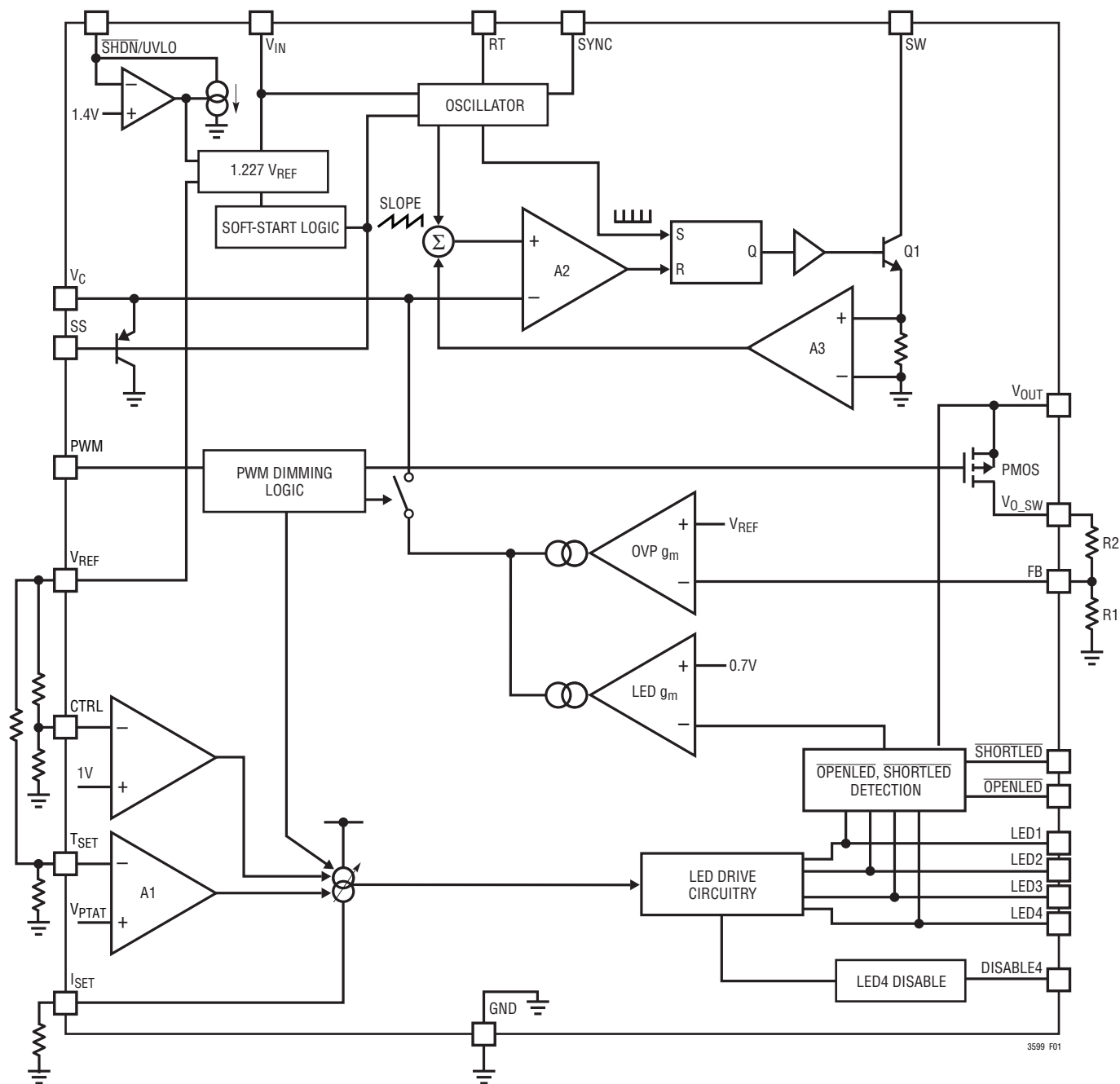
Figure 1. Block Diagram
