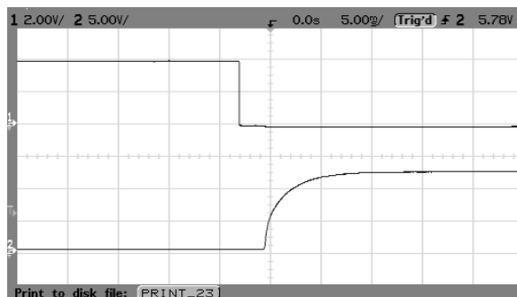
Fig. 70 AVO75-48S12 typical start-up from CNT on
