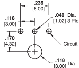
Recommended PC Board Layout 3 Position*
