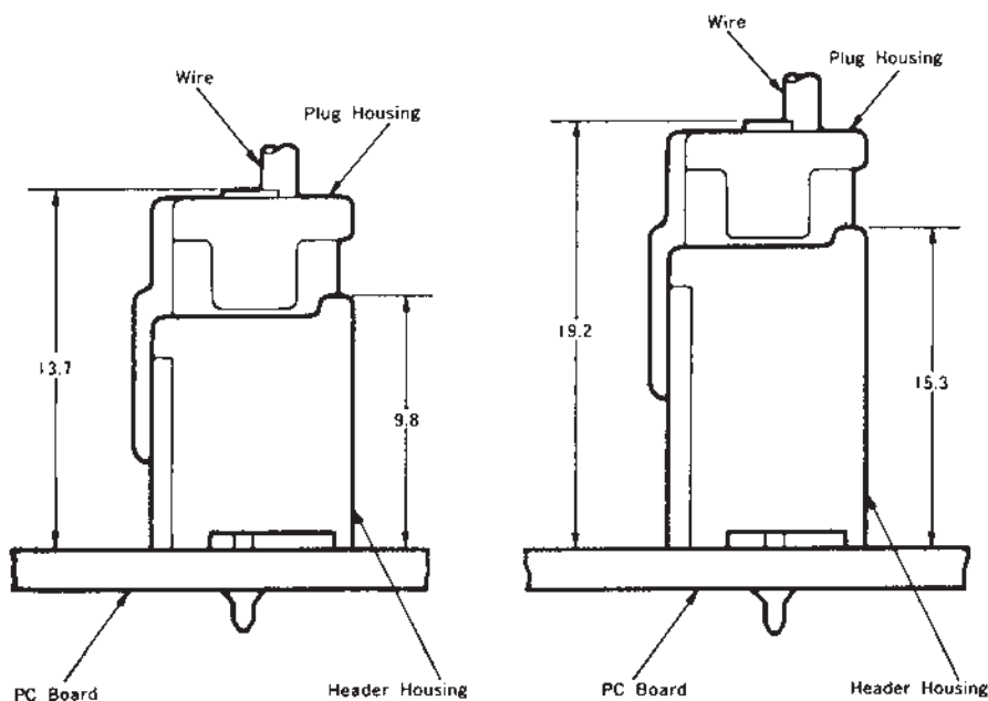
Standard-Profile Type
