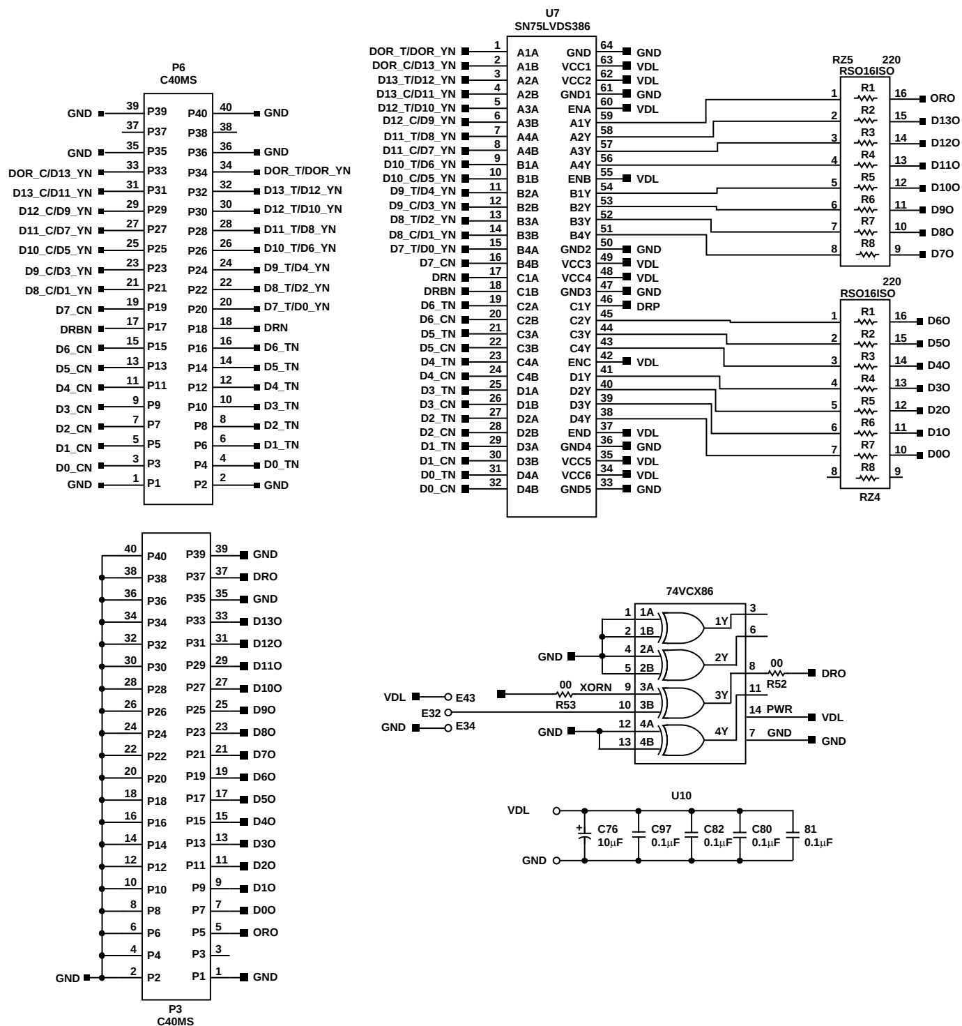
Figure 50. LVDS Mode Evaluation Board Schematic (Continued)
