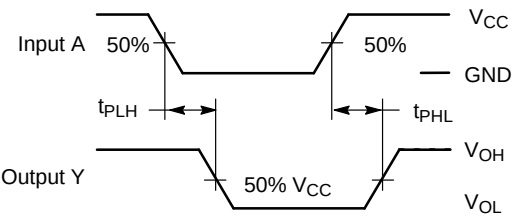
Figure 5. Switching Waveform
