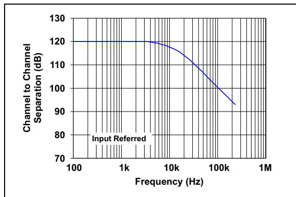
FIGURE 2-19: Channel-to-Channel Separation vs. Frequency (MCP6H92 only).
