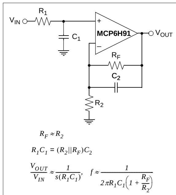
FIGURE 4-10: Non-Inverting Integrator.
