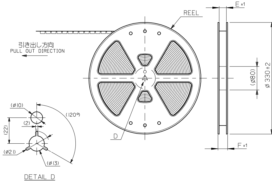
DETAIL D
