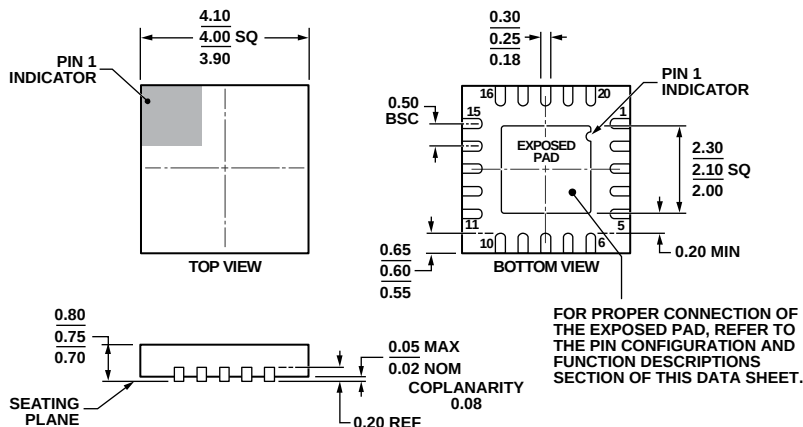
Figure 32. 20-Lead Lead Frame Chip Scale Package [LFCSP_WQ] 4 mm x 4 mm Body, Very Very Thin Quad (CP-20-6)
