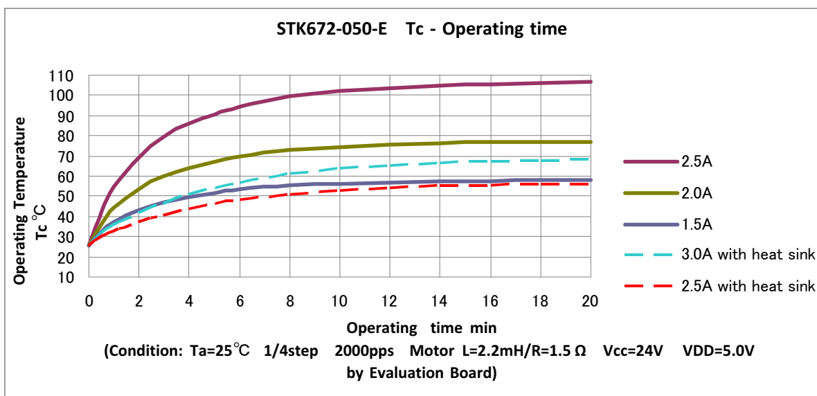
Figure 7. Operating Temperature
