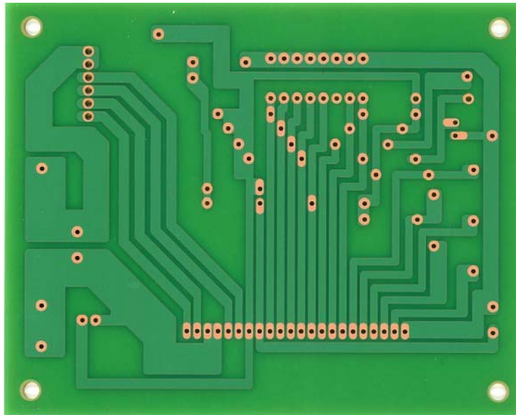
Figure 4. Copper Side (35 \mu )
