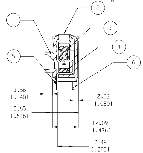
SECTION Z-Z
