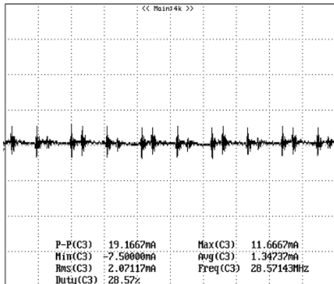
Figure 13: Input reflected ripple current, i_s , through a 12 \mu H source inductor at nominal input voltage and rated load current (20 mA/div, 20 ns/div).
