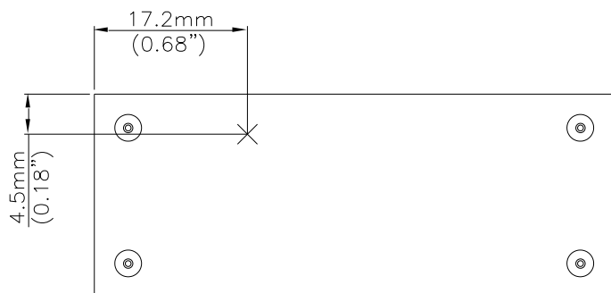
Figure 24: Hot spot 2's temperature measured point.
