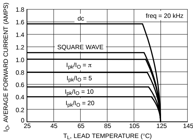
Figure 5. Current Derating
