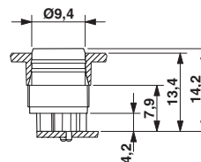
Dimensioned drawing
