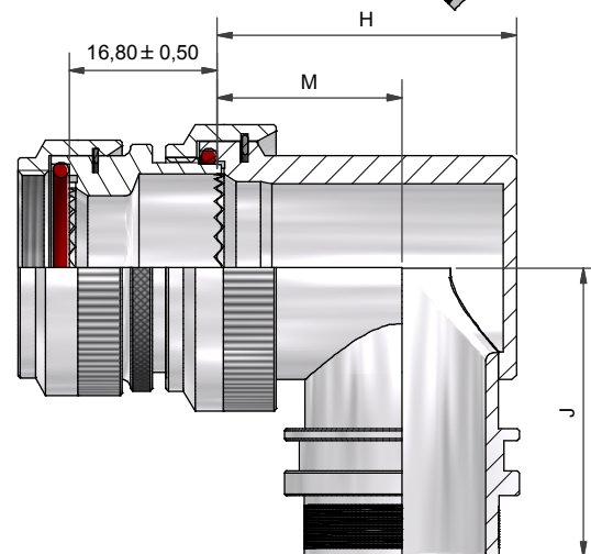
90° BACKSHELL - TYPE 2
