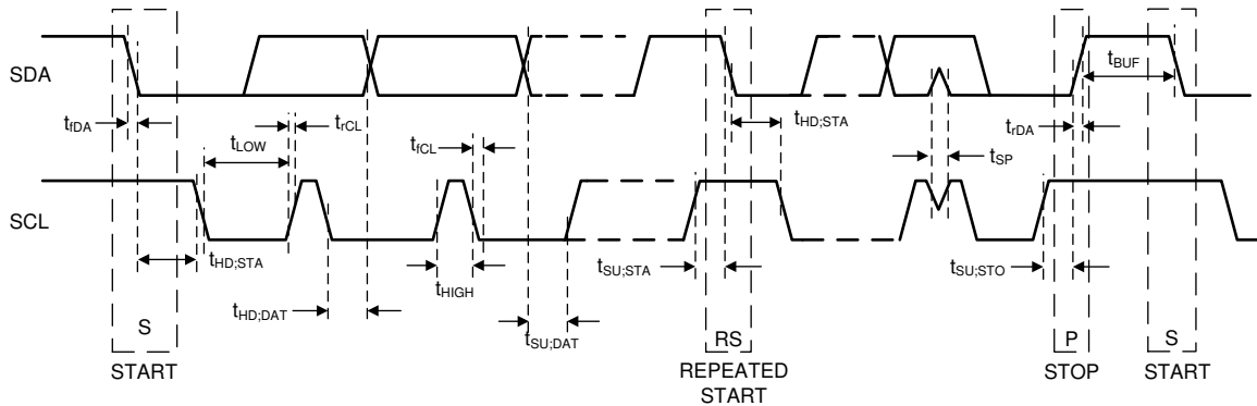
Figure 17. I²C-Compatible Timing
