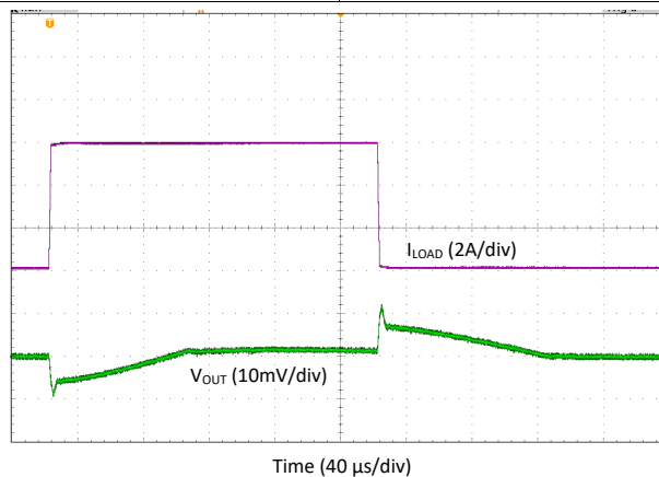
Figure 34. Transient Load Step Response, Forced-PWM-Four-Phase Mode, T_A = +25^\circ\text{C}
