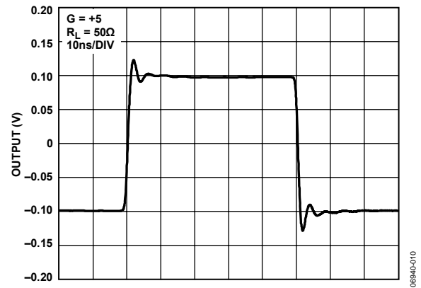
Figure 7. Small Signal Transient Response
