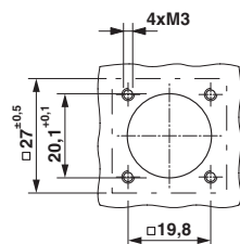
Installation dimensions
