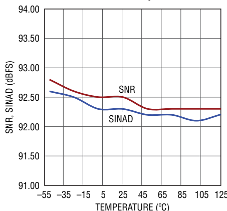
SNR, SINAD vs Temperature
