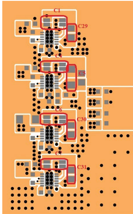
Figure 5. Split Pads for Output Capacitors on Top Layer of DC2637A
