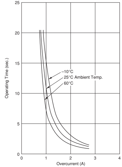
PTGL10AR3R9M3P51B0
