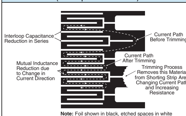
FIGURE 3 - TRIMMING TO VALUES (Conceptual Illustration)
