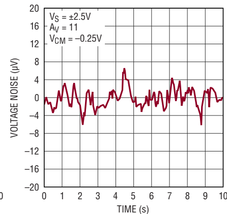
0.1Hz to 10Hz Input Referred Voltage Noise
