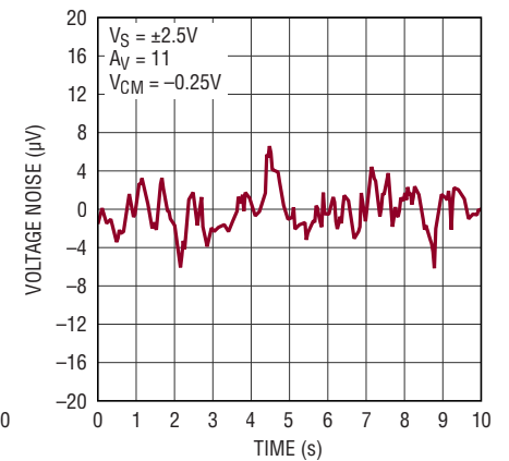
0.1Hz to 10Hz Input Referred Voltage Noise
