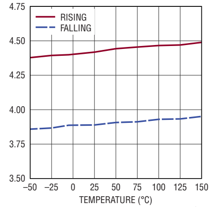
DRV CC UVLO Threshold vs Temperature
