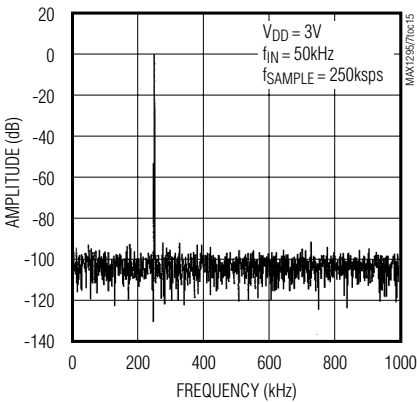
FFT PLOT
