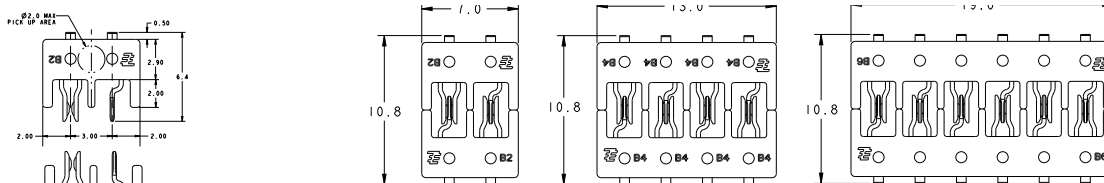
2, 4 and 6 position showing 2 mated parts
