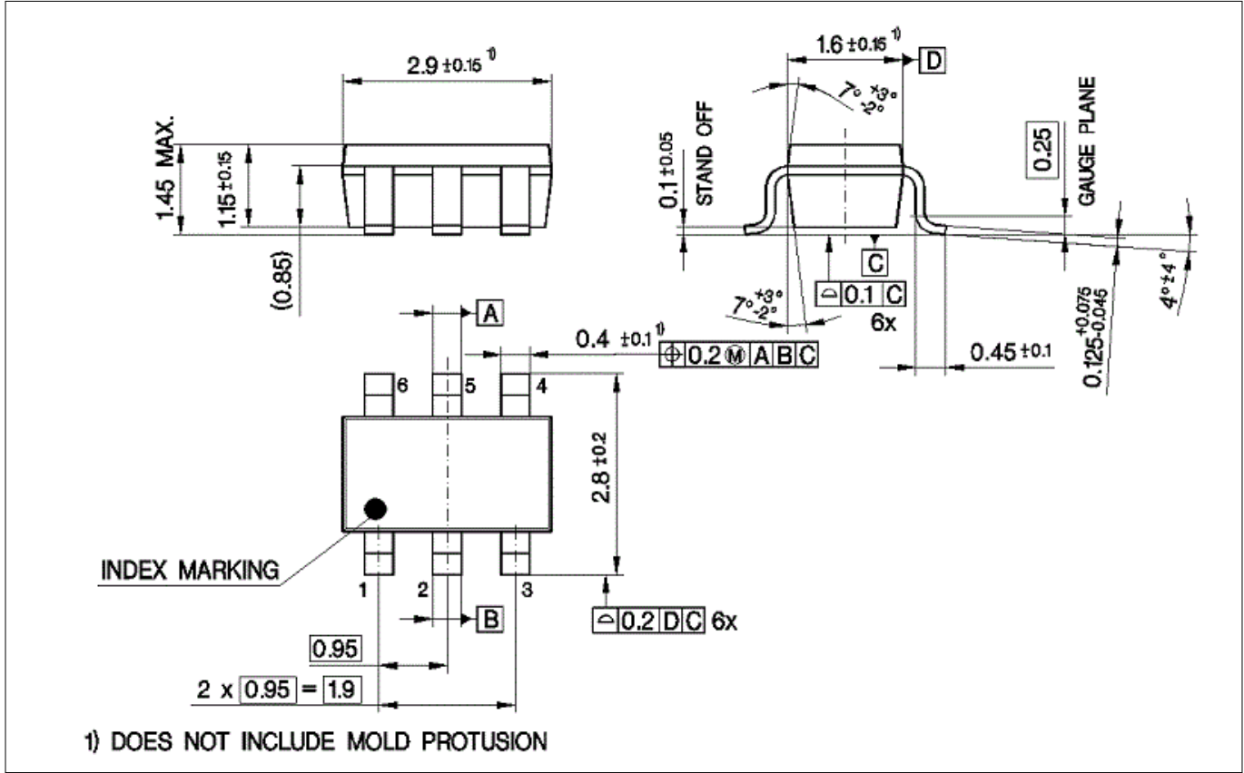
Figure 5 Package Drawings
