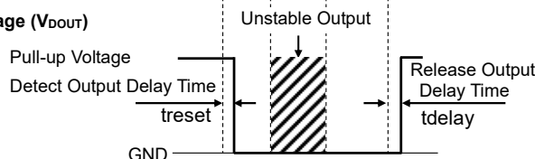
Operation Diagram
