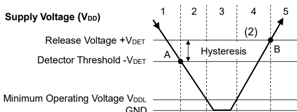
Output Voltage ( V_{DOUT} )
