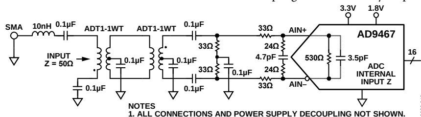
Figure 51. Differential Transformer-Coupled Configuration for Baseband Applications up to 150 MHz
