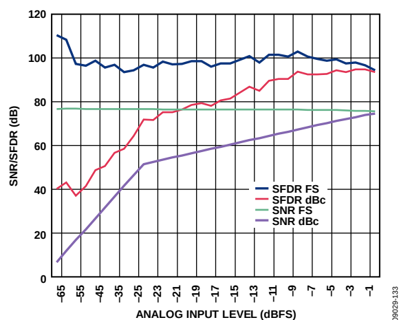
Figure 33. SNR/SFDR vs. Analog Input Level, f_{IN} = 97.3 MHz, 2.5 V p-p FS, AD9467-250
