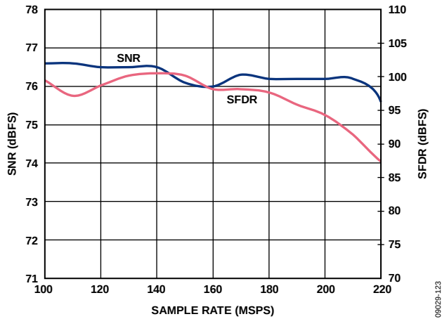
Figure 22. SNR/SFDR vs. f_{\text{SAMPLE}} , f_{\text{IN}} = 97.3 \text{ MHz} , 2.5 \text{ V p-p FS} , AD9467-200
