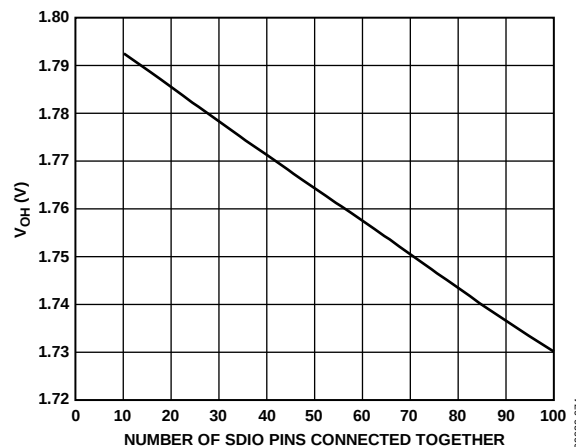
Figure 67. SDIO Pin Loading
