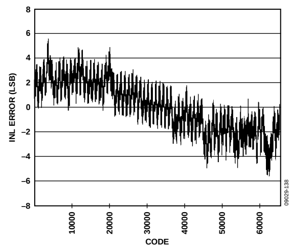
Figure 38. INL, f_{IN} = 4.3 MHz, 2.5 V p-p FS, AD9467-250
