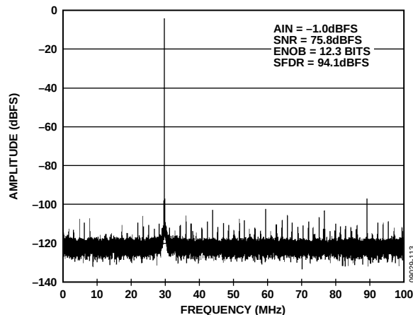
Figure 13. Single-Tone FFT with f_{IN} = 170.3 MHz, 2.5 V p-p FS, AD9467-200
